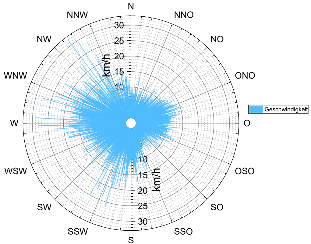
Wind-Maximum August 2026
