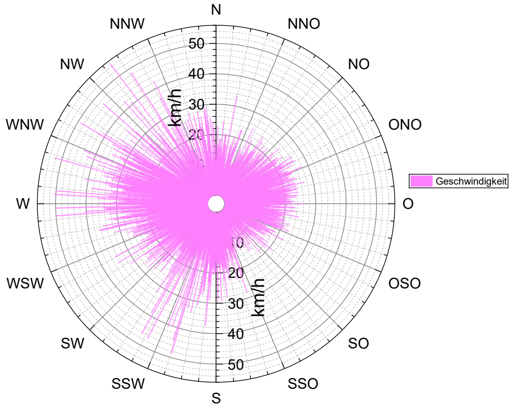
Böen-Maximum August 2026
